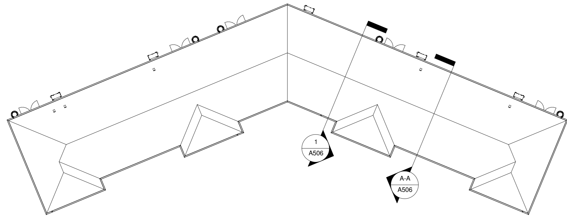
Section Location Plan 1 : 200
