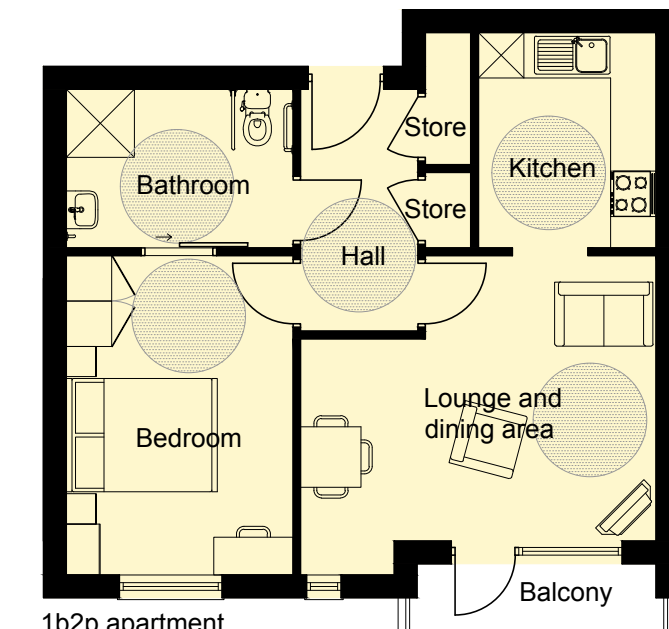
1b2p apartment 50.8m 2 /547ft 2 Apartment plans scale 1:100
