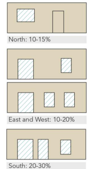
Recommended glazing percentages of each external facade
