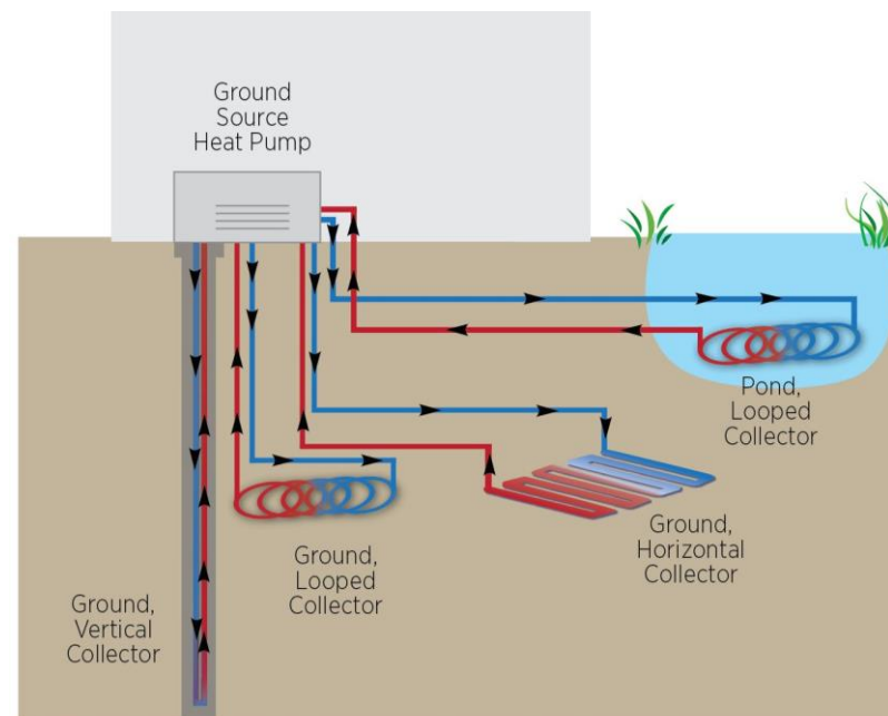
Different types of ground loop can serve the heat pump depending on the space available.
